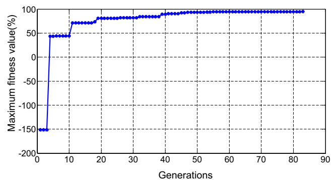
Fig. 8. Maximum fitness value in each generation of GA.
