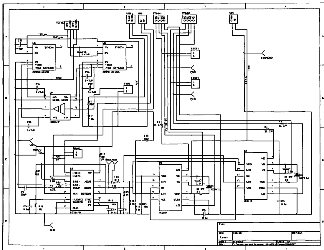
Fig. 3 The gate driver circuit design
