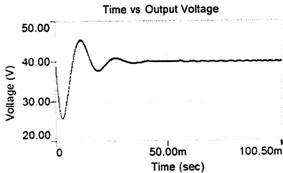
Fig. 5 Simulated output of the bidirectional converter with PID control
