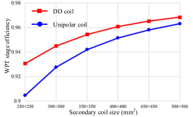
Fig. 14. WPT stage efficiency versus secondary coil size.
