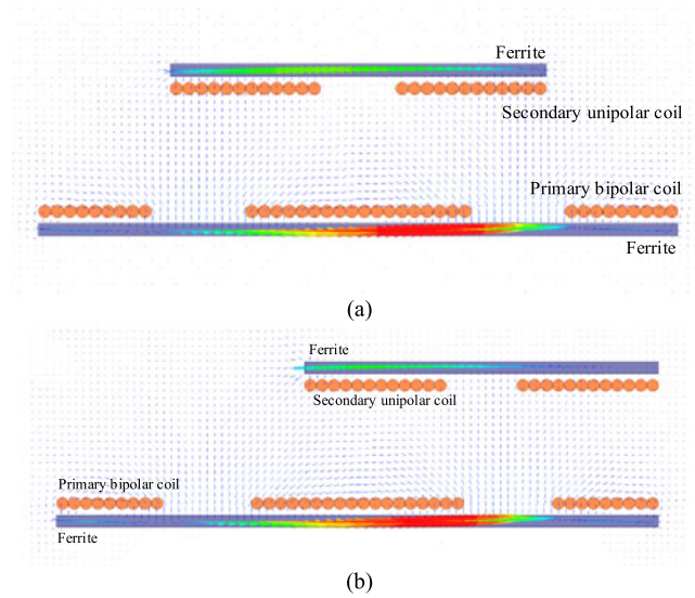
Fig. 19. Sketch to illustrate the magnetic field distribution of interoperability.
