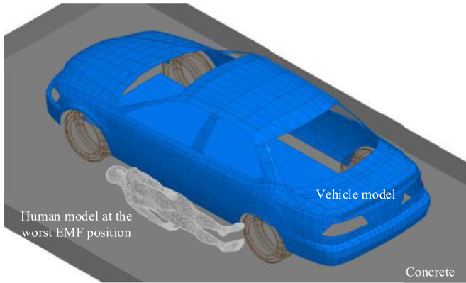
Fig. 20. Simulation models for radiation.
