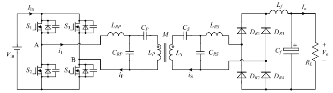
Fig. 24. LCC-LCC circuit diagram for experimentation.
