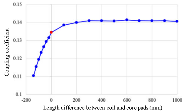
Fig. 2. Coupling coefficient versus the length difference between coil and magnetic core pads.
